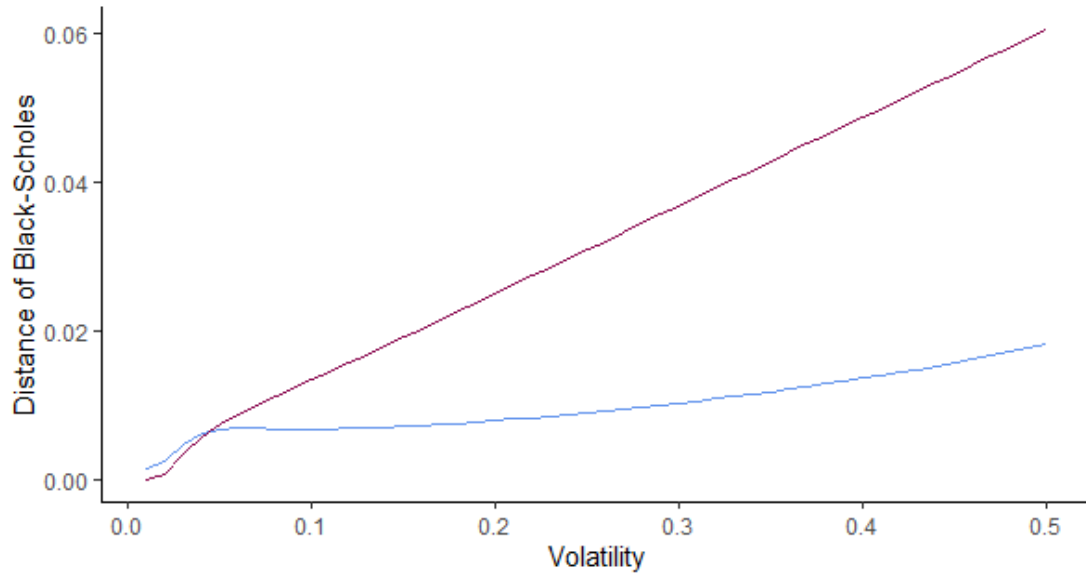
Volatility Analysis European Put
